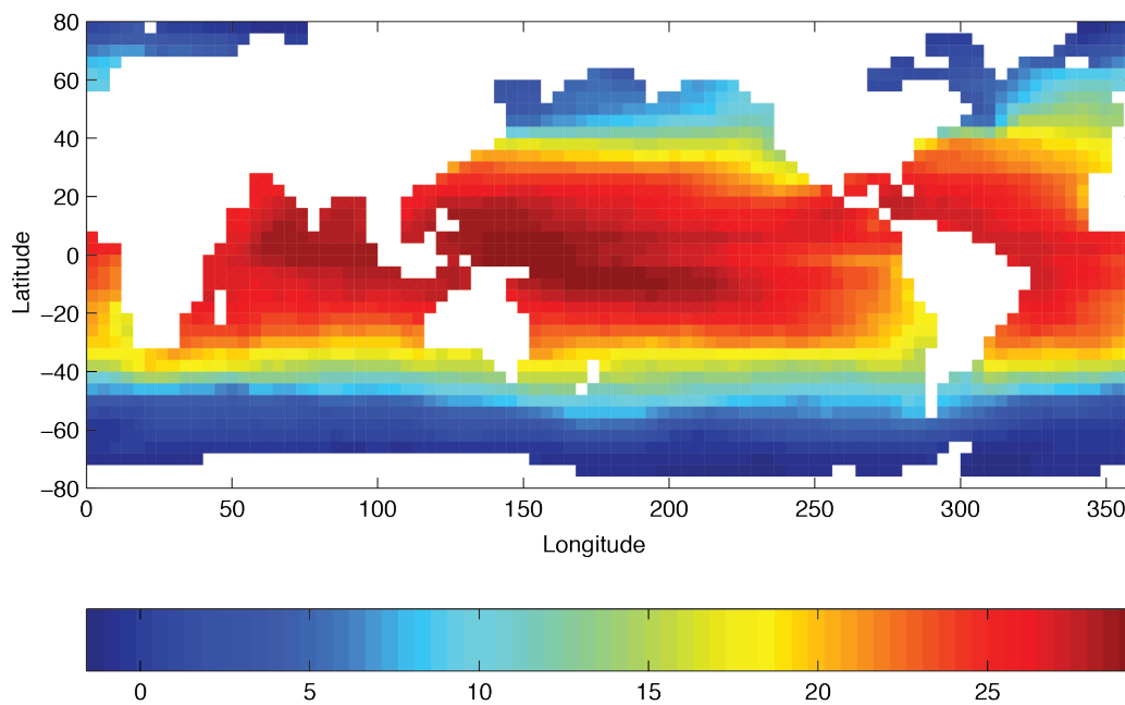
Figure 4.18: Annual mean of relaxation temperature ( ^{\circ}\text{C} )
