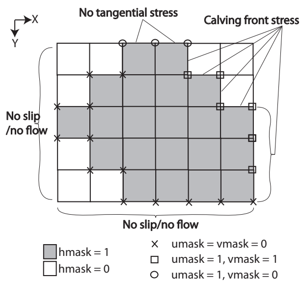
Figure 8.13: Hypothetical configuration, detailing the meaning of thickness and velocity masks and their role in controlling boundary conditions.
