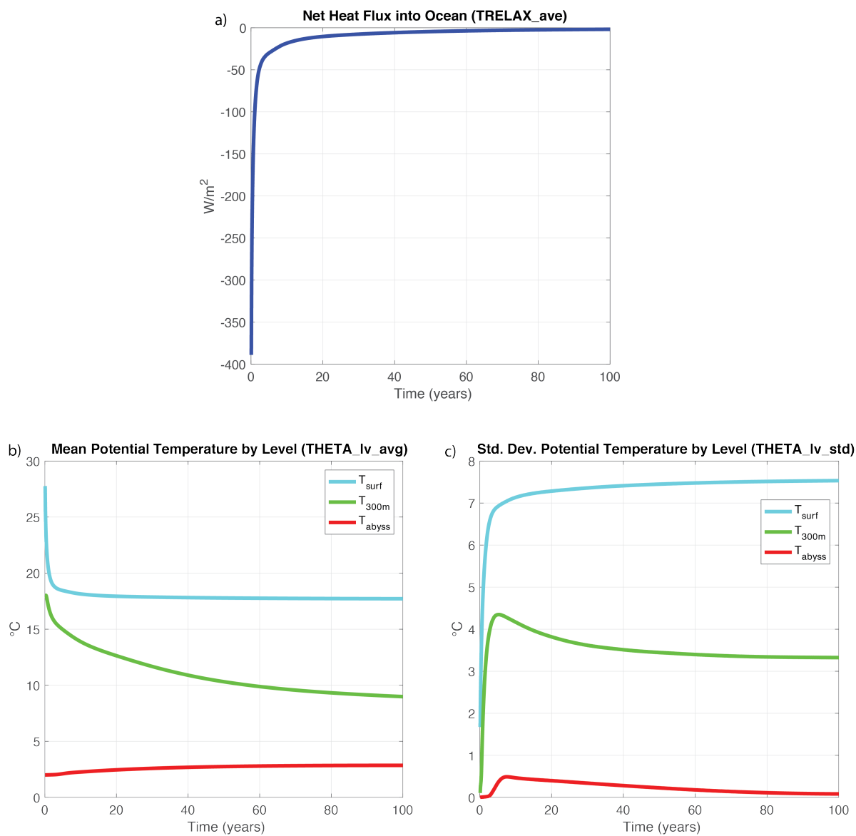
Figure 4.6: a) Surface heat flux due to temperature restoring, negative values indicate heat flux out of the ocean; b) and c) potential temperature mean and standard deviation by level, respectively.
