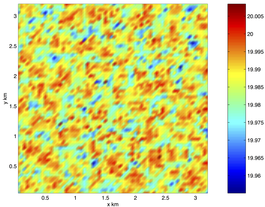
Figure 4.27: Surface section
